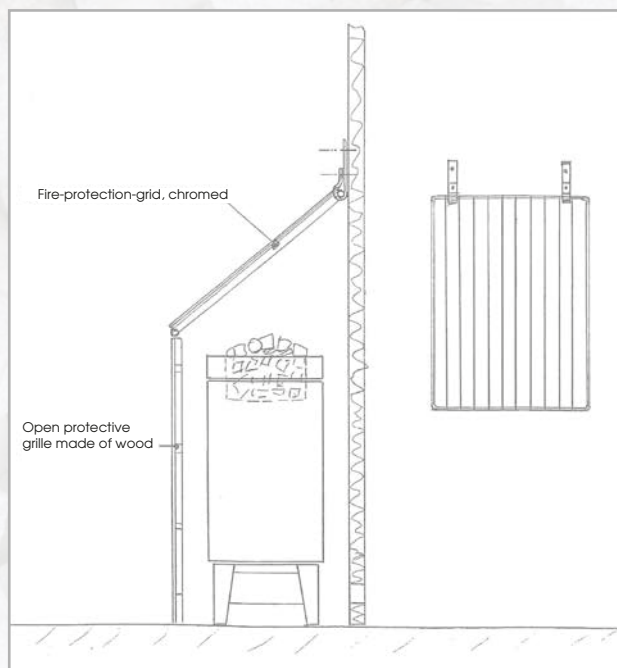
Figure: Fire-protection-grid, chromed with 2 fixing clamps.
